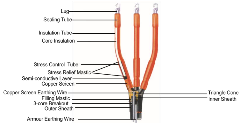
10KV Indoor Heat Shrinkable 3-core Termination
